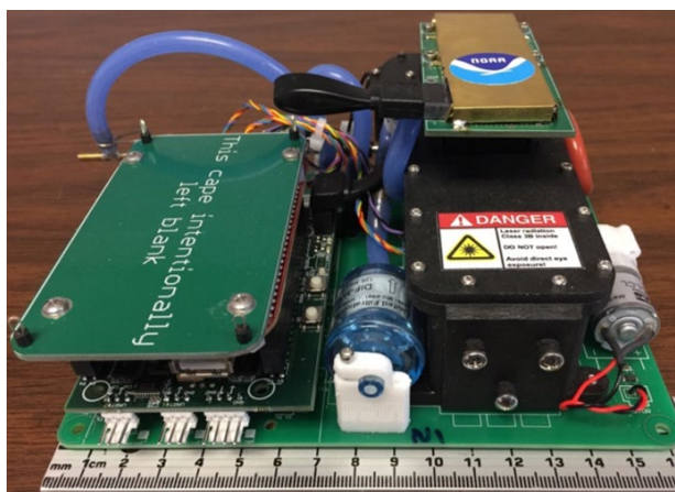
NOAA CSL's Portable Optical Particle Spectrometer (POPS) uses an on-board laser to measure tiny suspended particles that influence stratospheric chemistry and reflect incoming sunlight. The miniaturized instrument, designed by CSL researchers in Boulder, Colorado, weighs 1.3 pounds and is about the size of a lunch box. Credit: NOAA
