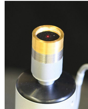
Close-up of a microphone, with the laser spot hitting the center of its diaphragm. Credit: NIST
