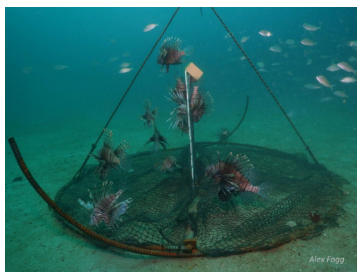
A lionfish trap undergoes scientific testing in the Gulf of Mexico.
