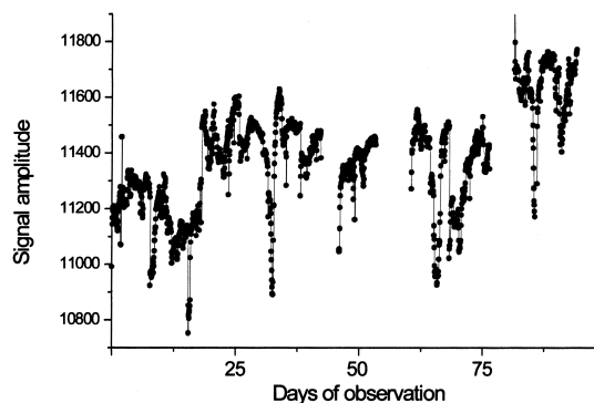
Fig. 1. Variations with time of the EPR signal of a stable paramagnetic material permanently present in the cavity of an older Bruker ESP300 spectrometer. Signal-to-noise ratio was greater than 10,000:1. Microwave power: 0.25 mW, modulation amplitude: 0.5 mT.
