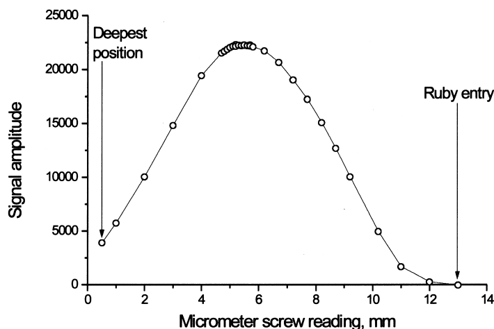
Fig. 4. Dependence of the amplitude of the ruby line at 220 mT on the readings of the micrometer screw of the ruby holder. Bruker cavity 4103TM with the standard quartz tube for alanine pellets (O. D. 7 mm; I. D. 5 mm).
