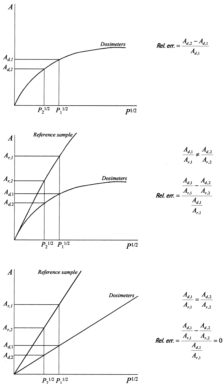
Fig. 5. Magnitude of the errors due to microwave power variations. Top: No adjacent reference sample used; no correction for signal change as a result of the power decrease from P_1 to P_2 . Middle: An adjacent reference sample is used, but the signals are partly saturated; a partial correction for the power decrease. Bottom: The power is low enough, so that none of the signals is saturated; a perfect correction for the power decrease.
