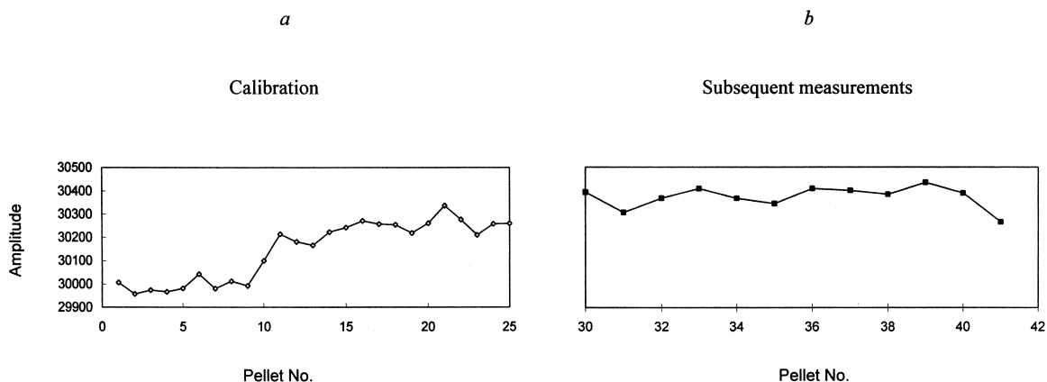
Fig. 10. Amplitudes of the signals of a ruby adjacent reference sample in the course of dose measurements for a custom source calibration. The pellet numbers show the order of recording the spectra.
