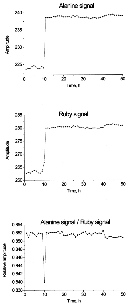
Fig. 12. Incomplete correction in the case of a very sharp change in the spectrometer sensitivity.
