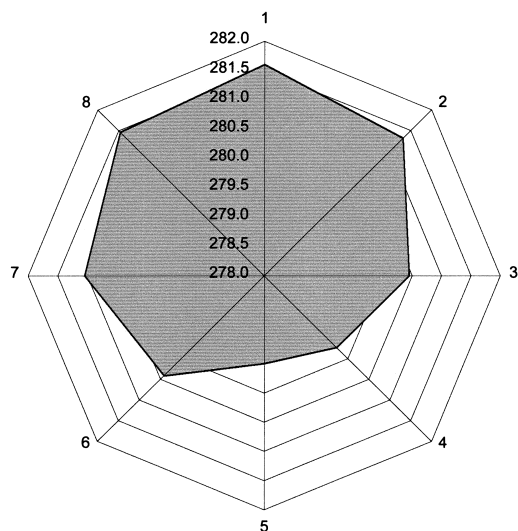
Fig. 8. Dependence of the ruby signal amplitude on the orientation of a quartz tube holder in a 4103TM cavity. Polar coordinates are used: numbers 1–8 designate eight tube orientations spaced by 45° the radial distance from the center shows the ruby signal amplitude.
