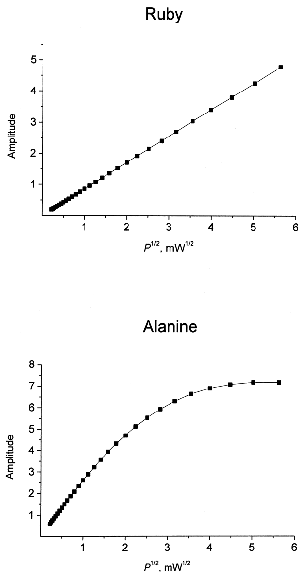
Fig. 6. Dependence of the amplitudes of the signals of the ruby reference sample and alanine on microwave power. ECS106, cavity 4103TM with the standard quartz tube for dosimeters; the ruby crystal is located near the front wall.
