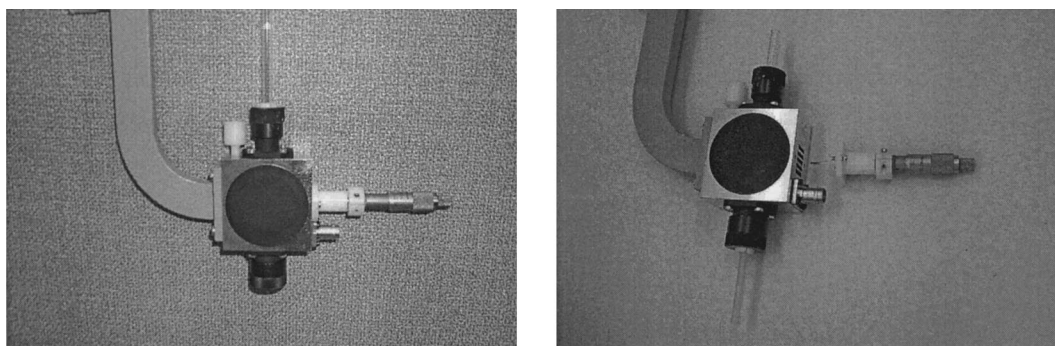
Fig. 2. Adjacent reference sample device manufactured by Bruker Instruments. Left: Assembled cavity with the reference sample device attached and quartz holder for alanine pellets. Right: The same construction in the disassembled form; the dark ruby rod and the illumination grid used for its insertion can be seen.
