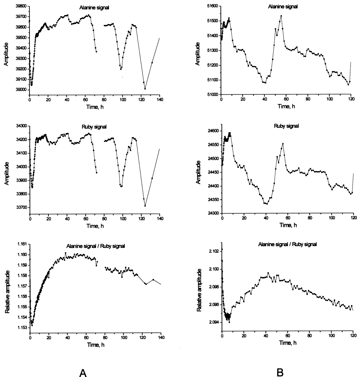
Fig. 9. Effect of normalization to the signal of the adjacent ruby reference sample in studying evolution of the alanine signal after ^{60}\text{Co} gamma irradiation. A 50 kGy; B 100 kGy.
