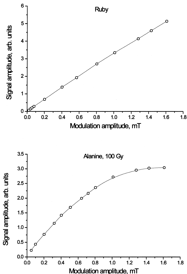
Fig. 7. Dependence of the amplitudes of ruby and alanine signals on modulation amplitude. Least-squares fit for the alanine dependence in the range 0.05–0.8 mT: Y = 0.474 + 3.877x - 1.252x^2 + 0.000413x/\ln x ; standard error of the fit is 0.012.
