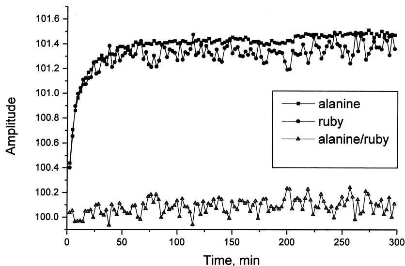
Fig. 11. Changes in the amplitudes of alanine and ruby signals, as well as in their ratio, for a dosimeter just brought in from an environment with a relative humidity higher than the humidity of the EPR laboratory.
