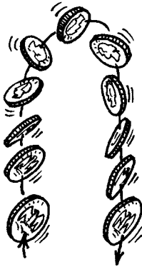
FLIPPING A COIN IS ONLY AN ILLUSION OF RANDOMNESS IN NEWTON'S WORLD.
